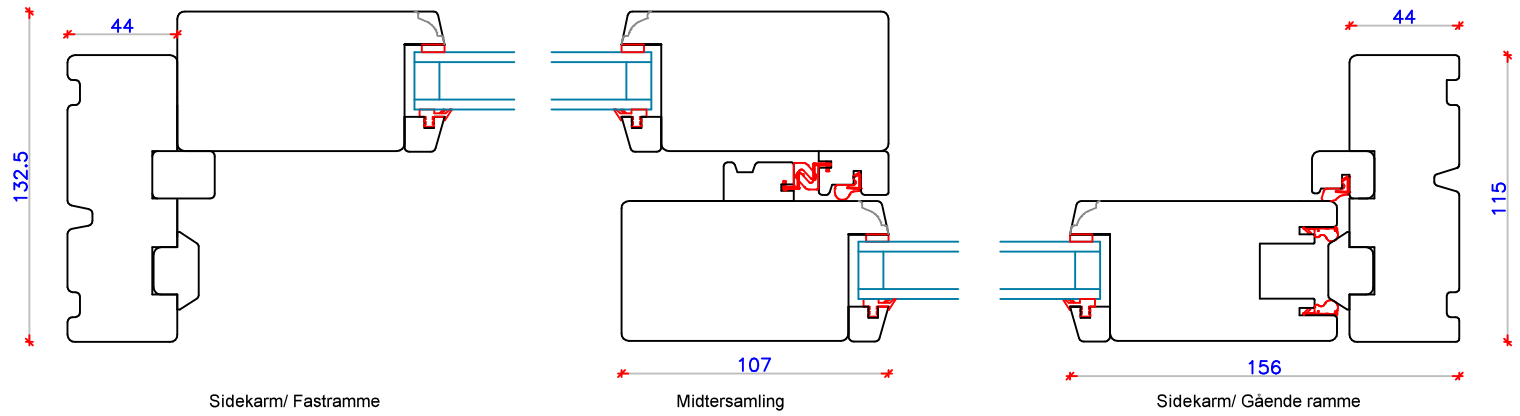
Sidekarm/ Fastramme
